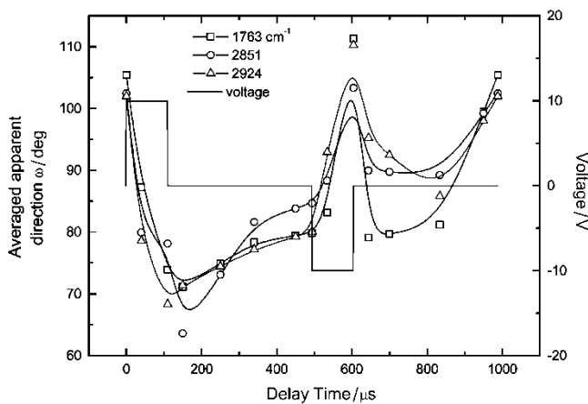
Figure 12. Transient orientations of several molecular segments associated with the C=O moiety and alkyl chain are presented as a function of delay time. The solid lines are a guide for the eye.
